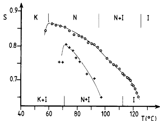
Figure 9. Temperature dependence of order parameter of DDA9. Key: O, neat DDA9; +, DDA9 in mixture.
