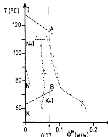
Figure 11. Temperature dependence of \phi_N^M and \phi_I^M in the DDA9-NBd5 mixture. The phase diagram is delineated by the dashed lines. Note the broad N + I biphasic of pure DDA9, strongly broadened by addition of small amounts of NBd5. Point A is T_I of the 0.07 mixture. Point B is the appearance of the crystallization of the 0.07 mixture. The two lines going through the black points ( \phi_N^M and \phi_I^M ) are not part of the phase diagram, but represent the NBd5 mass fraction in the N (or K) component (left) and the I component (right) of the biphasic in the 0.07 mixture.
