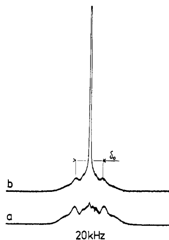
Figure 6. 1 H NMR spectra of DDA9. (a) neat DDA9 at 91 °C; (b) in mixture with 7.4% NBd5 at 78 °C. Note the sharp peak corresponding to the I component of the biphasic.
