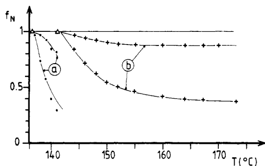
Figure 4. Temperature dependence of nematic fraction f_N in the N + I biphasic. (a) 0.07 mixture; (b) 0.15 mixture. Upper curves refer to PTFC ( f_N^H ). Lower curves refer to PAA14 ( f_N^D ).
