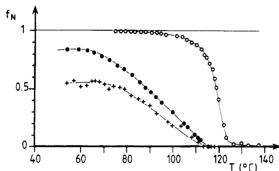
Figure 8. Temperature dependence of the nematic fraction, f_N . Key: O, pure DDA9, f_N^H ; ●, DDA9 in mixture, f_N^H ; +, NBd5 in mixture, f_N^D .
