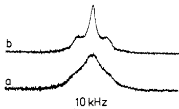
Figure 2. ^1\text{H} NMR spectra of neat PTFC. (a) 120 °C; (b) 160 °C.
