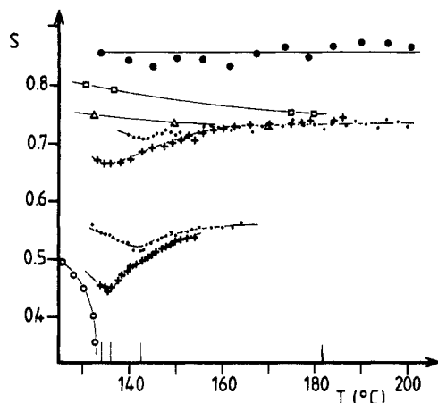
Figure 3. Temperature dependence of order parameters. Key: ●, neat PTFC; □, PTFC in 0.45 mixture; △, PTFC in 0.30 mixture; •, top PTFC in 0.15 mixture, bottom PAA14 in 0.15 mixture; +, top PTFC in 0.07 mixture, bottom PAA14 in 0.07; ○, neat PAA14. Vertical bars (from left to right): T_{NI} of PAA14; T_N of 0.07, 0.15, and 0.30 mixtures. The 0.45 mixture did not reach N + I biphasic within experimental range.
