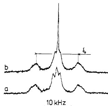
Figure 1. 1 H NMR spectra of PTFC in PAAAd14 (0.07 mixture). (a) pure N phase at 122.5 °C; (b) N + I biphasic at 138 °C. Note the sharp peak corresponding to the I component of the biphasic.
