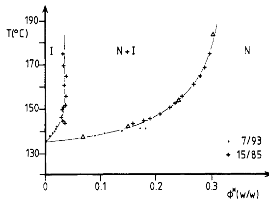
Figure 5. Phase diagram for the PTFC-PAA14 system. Key: •, from data for 0.07 mixture; +, from data for 0.15 mixture; △, experimental T_N values for the 0.07, 0.15, 0.24, and 0.30 mixtures.
