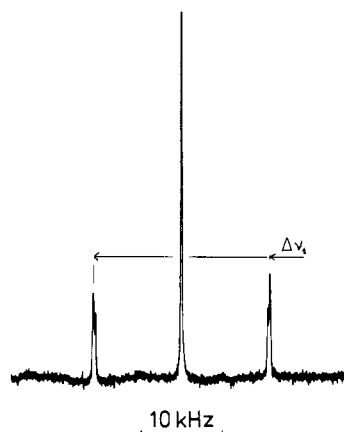
Figure 7. 2 H NMR spectrum of NBd5 in the 0.074 NBd5–DDA9 mixture at 87 °C. The sharp central peak corresponds to the NBd5 in the I component of the biphasic.
