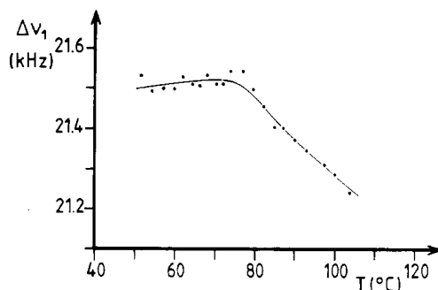
Figure 10. Temperature dependence of the quadrupolar splitting, \Delta\nu_1 , of NBd5 in the N component of the mixture.
